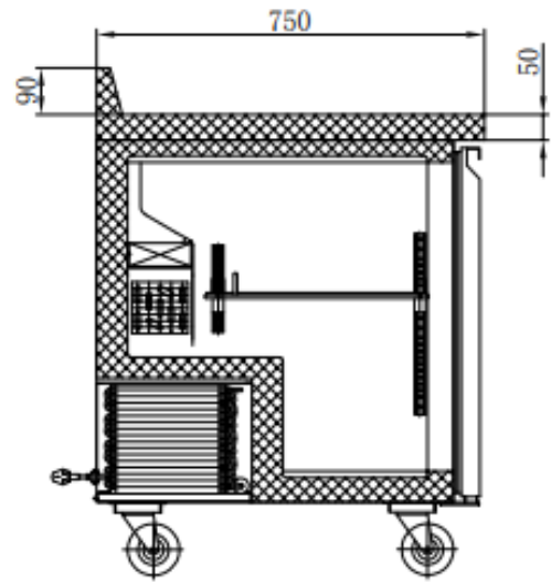
SECTION VIEW
